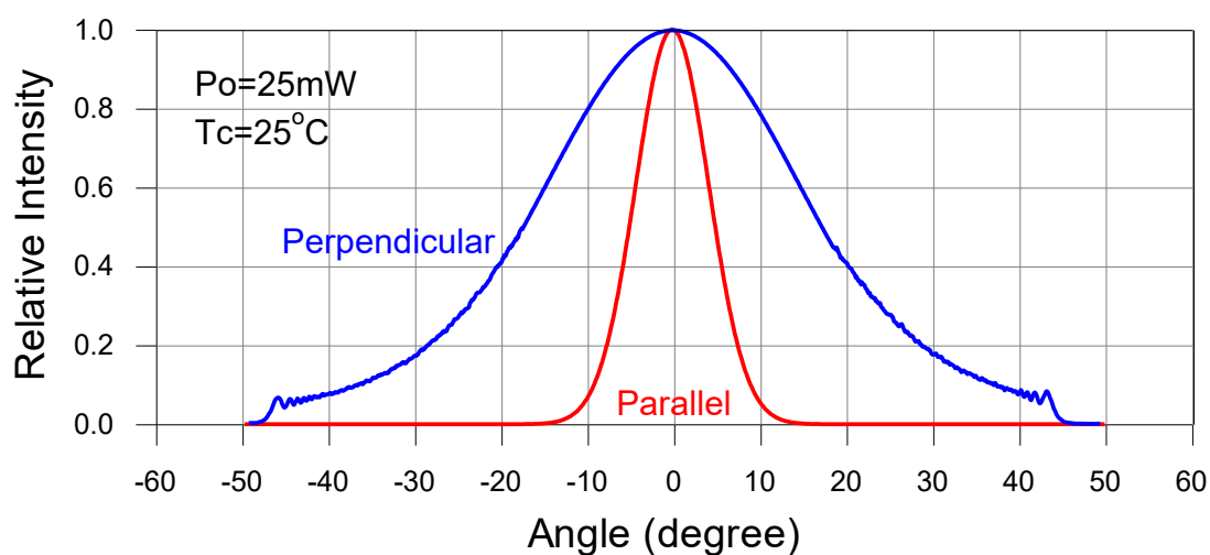
Far-Field Pattern
