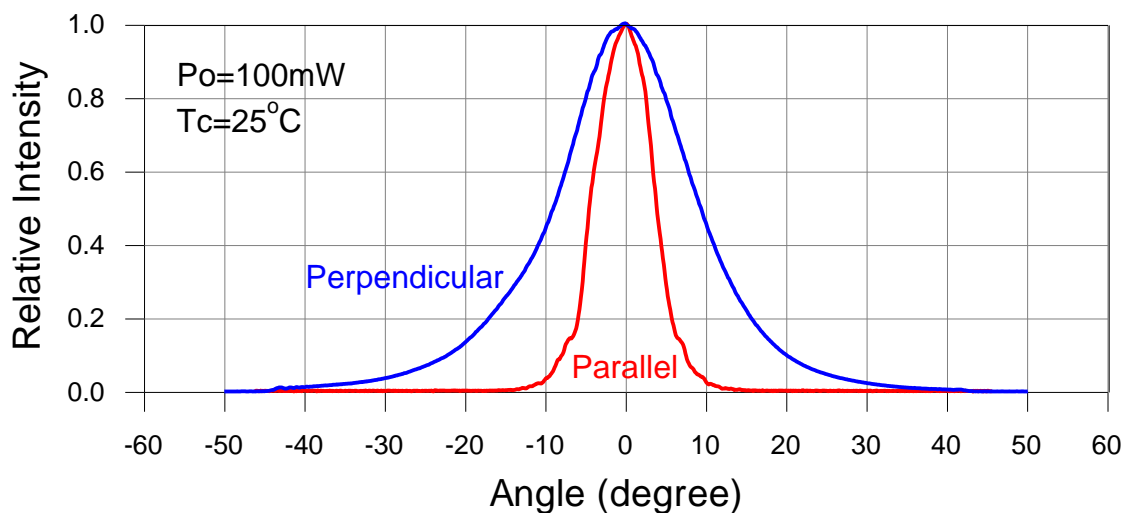
Far-Field Pattern
