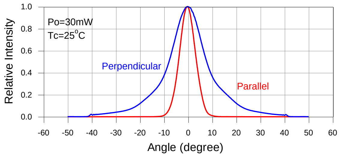
Far-Field Pattern
