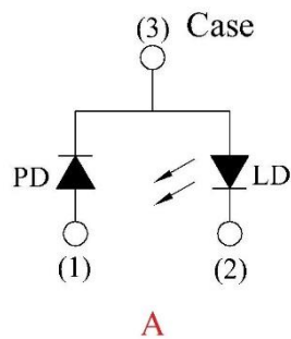
Pin configuration
